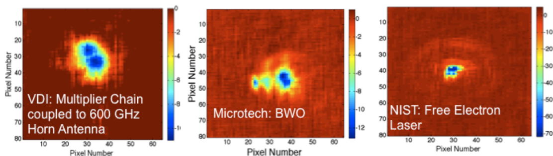
Fig. 3 Images of three THz sources collected with THEIA: (left) 600 GHz Virginia Diode Source, (center) Microtech backward wave oscillator source (680 GHz), (right) NIST Free Electron Laser.
